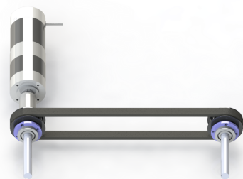
Figure 2: Drivetrain
