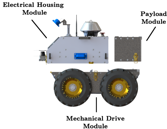
Figure 1: Hardware Modules
