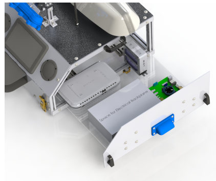
Figure 5: Module with drawer open
