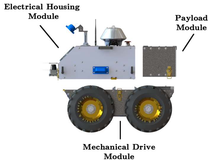
Figure 1: Hardware Modules
