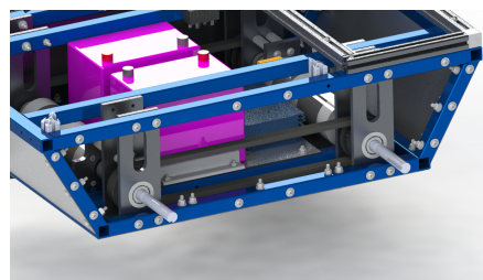
Figure 3: Side View
