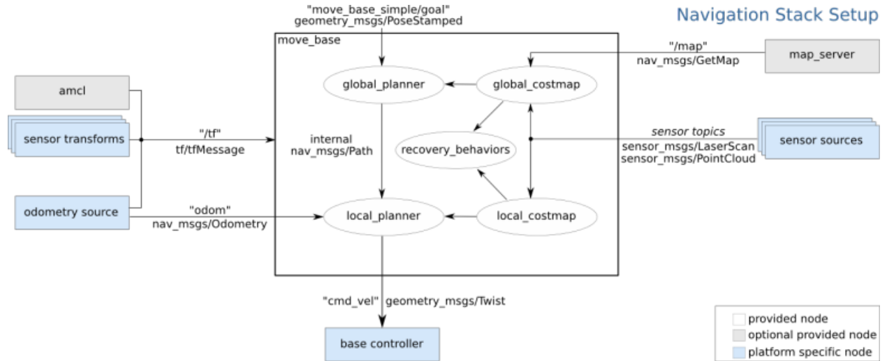
Figure 7: Navigation Stack Setup
