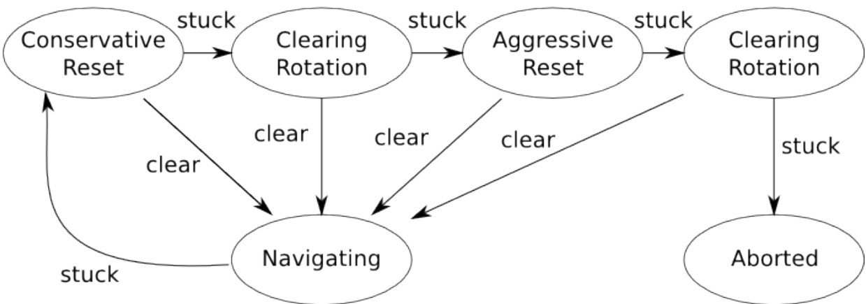
Figure 9: Recovery Behaviors
