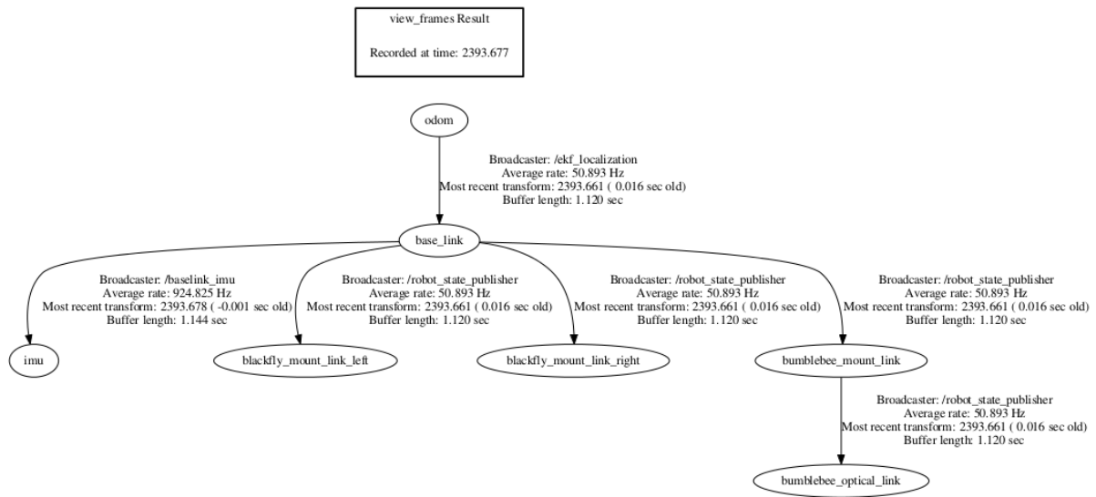
Figure 8: TF tree
